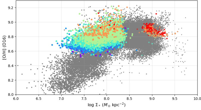
HII rMZR scatter (PG16)
