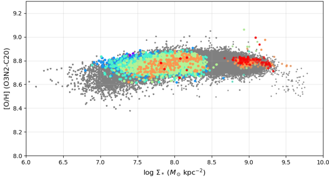
HII rMZR scatter (O3N2-C20)
